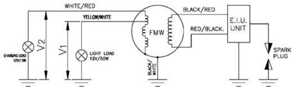
CIRCUIT DIAGRAM
